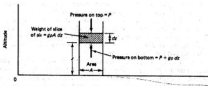
A column of air in static equilibrium used to determine the relationship between air pressure and altitude.
